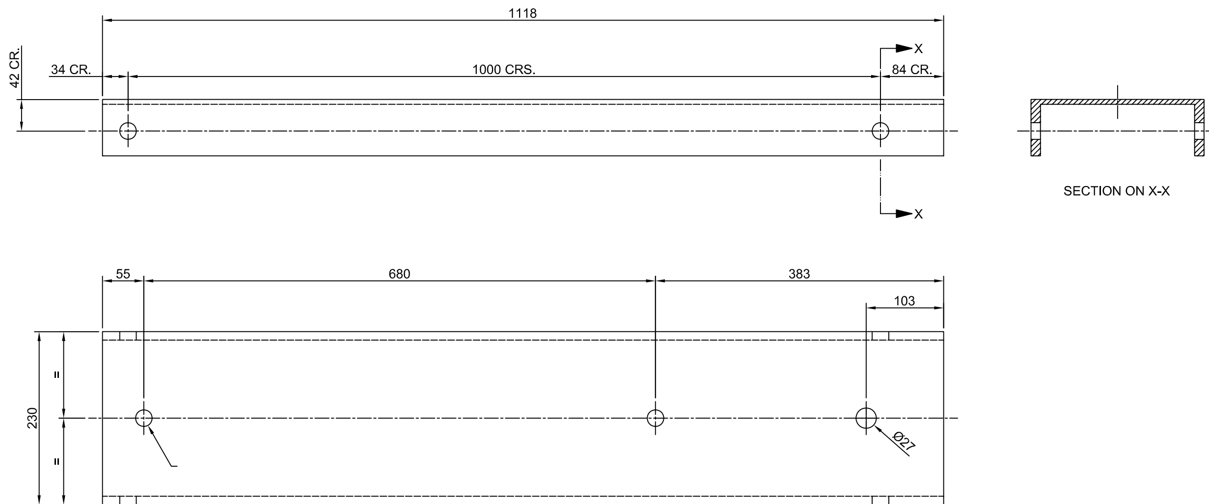
ITEM 5. 1118 x 230 x 75 (25.7 kg/m) PARALLEL FLANGE CHANNEL TO B.S. 4 PART 1: 1993.
